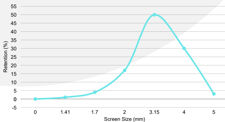
Typical Particle Size Retention of Precoat SBR 2-5
